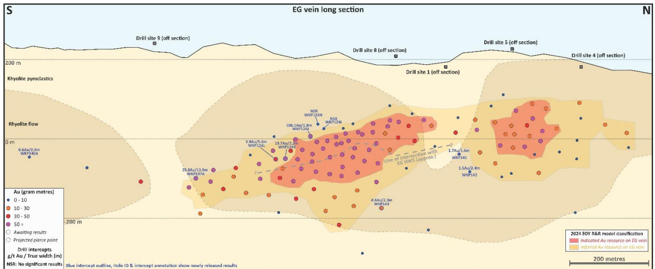
Figure 2: Long section of the EG vein with geology and drill intercepts (blue font = new holes)
