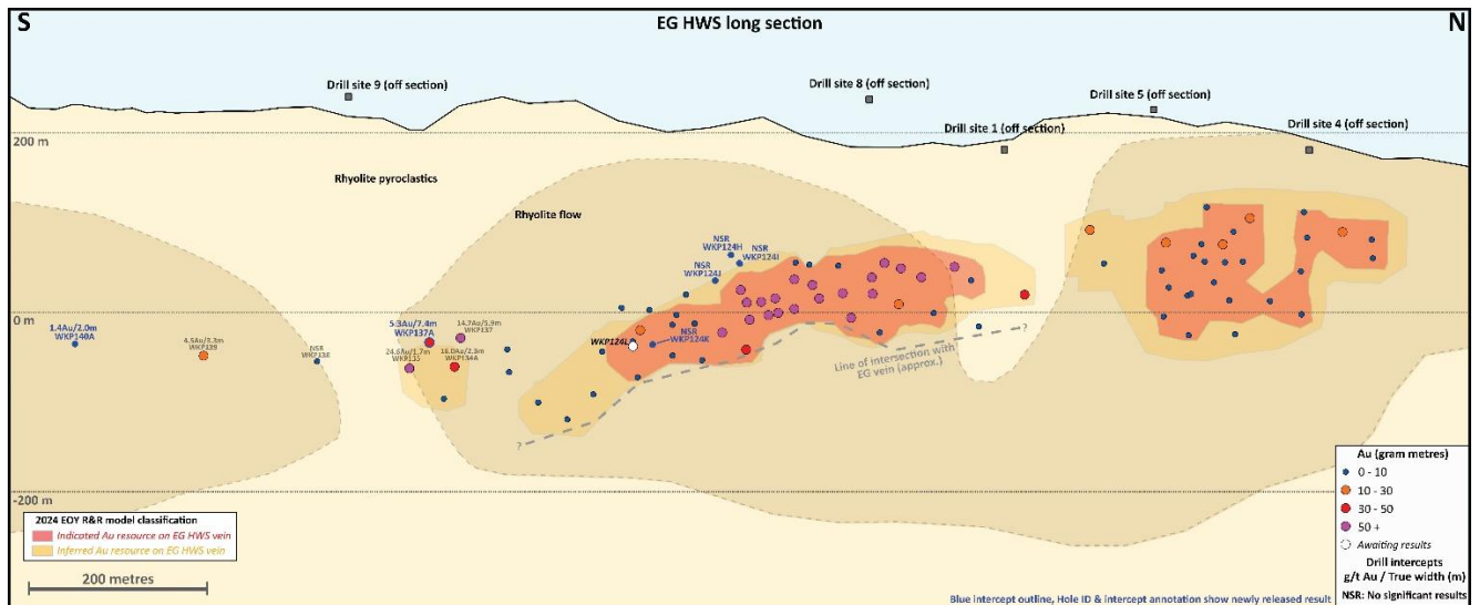
Figure 3: Long section of the EG HWS vein with geology and drill intercepts (blue font = new holes)
